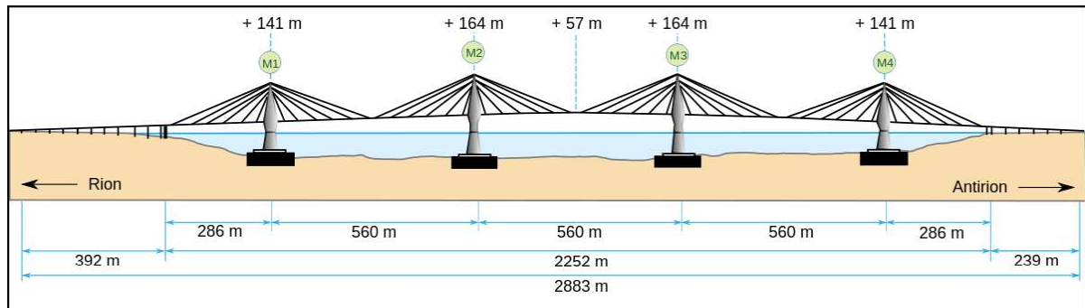
Fig. 1. General Layout of the bridge
