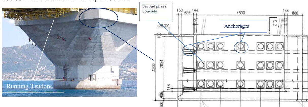
Fig.3. Pylon Base prestressing anchorage area
