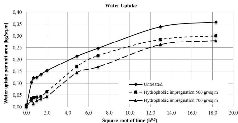
Fig. 7. Water uptake as a function of time
