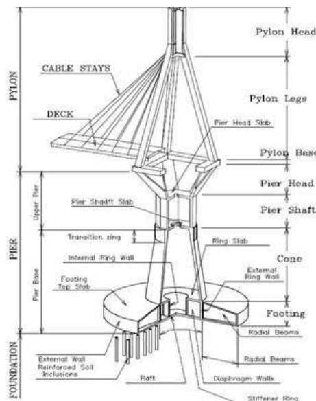
Fig.2. Topology of structural elements of the bridge
